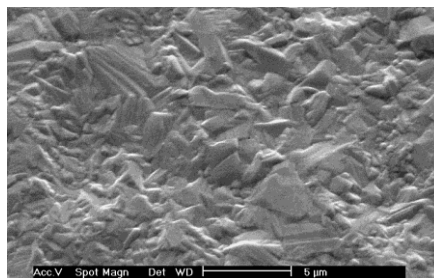
● Electrolytic Copper Foil Etched 1 μm by CPE-750
