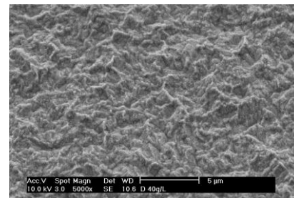
● Electrolytic Copper Foil Etched 1 μm by CPE-930
